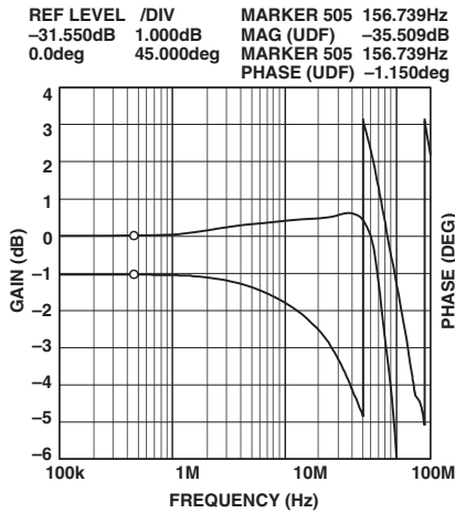
TPC 3. Frequency and Phase Response vs. Gain (Gain = +30 dB, P_{IN} = -30 dBm, Pin 5 Connected to Pin 7)
